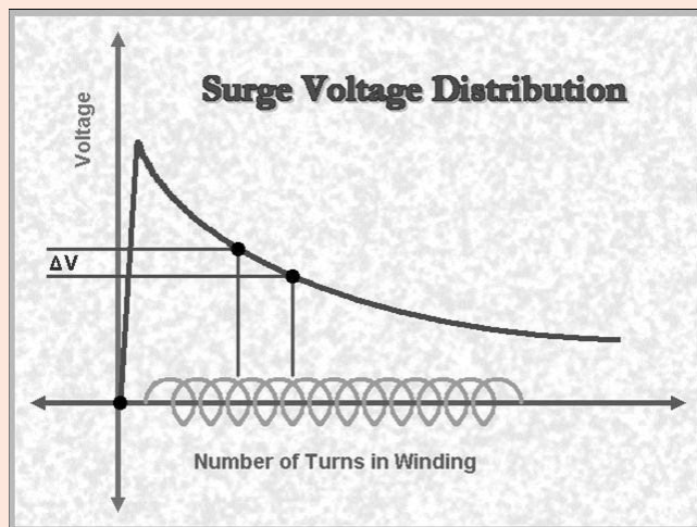
Figure 1: Initial impulse voltage distribution in a coil
