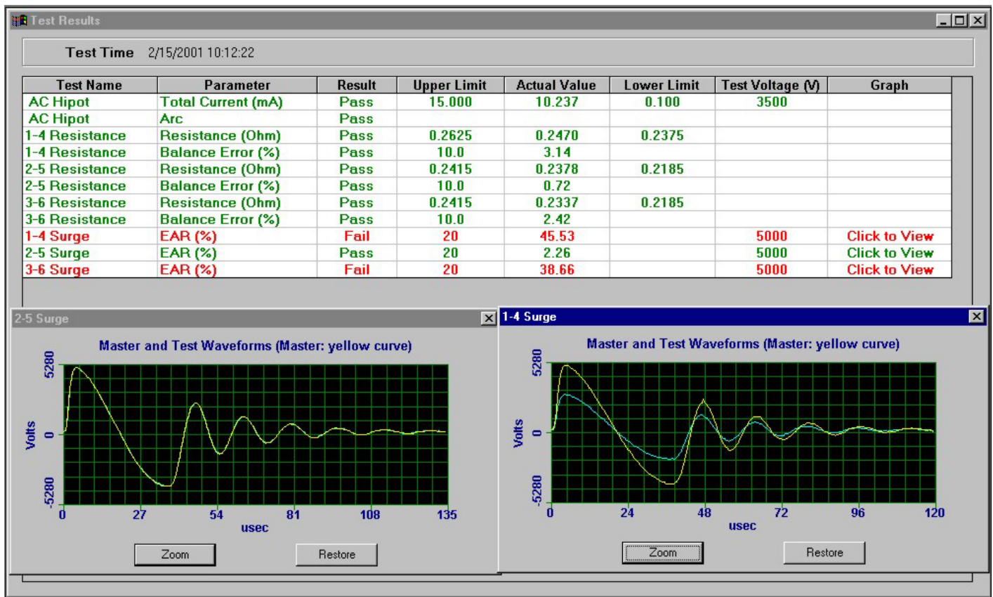
The WinAST rapidly compares multiple surge waveforms against a reference waveform for quality assurance testing of a given production motor.
