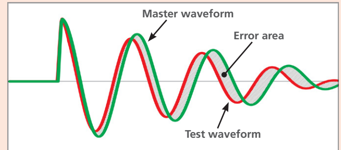
Figure 2: A mathematical percent error is calculated for the difference between a good and a shorted coil
