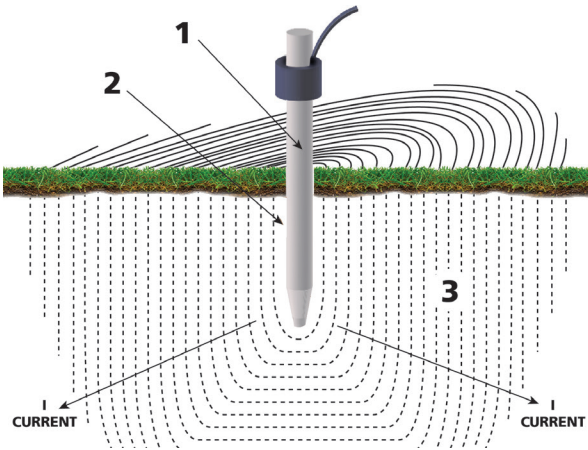
Fig. 9: Components of earth resistances in an earth electrode
