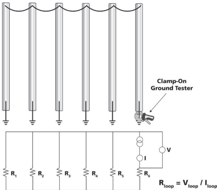
Fig 22: Pole ground application
