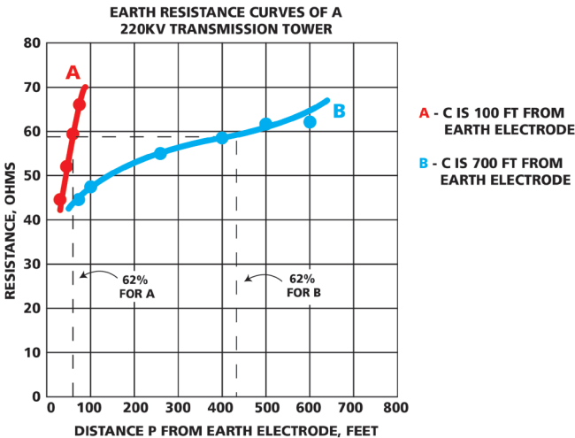
Fig. 14: Example of how C location affects the earth resistance curve
