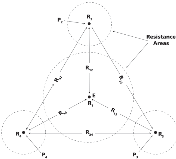
Fig 27: Star-Delta test configuration
