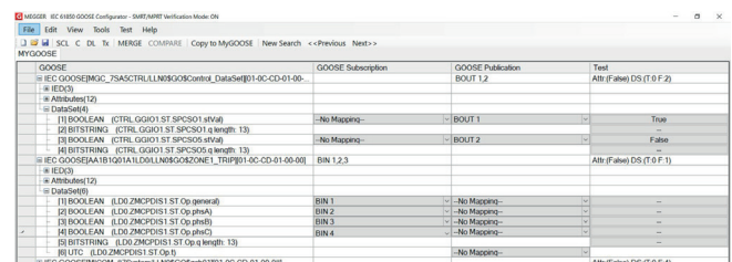
Figure 5: Megger GOOSE Configurator software
